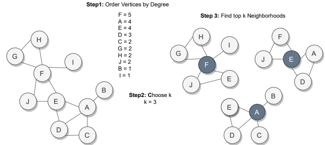
Fig. 3. Visualization of the high level steps of the TN-Neighborhoods algorithm.
