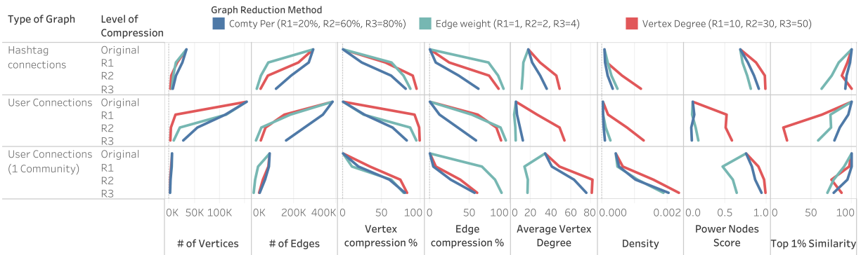
Fig. 8. Comparison of the different reduction techniques for three graphs of different sizes. Data was extracted from the Austin dataset.
