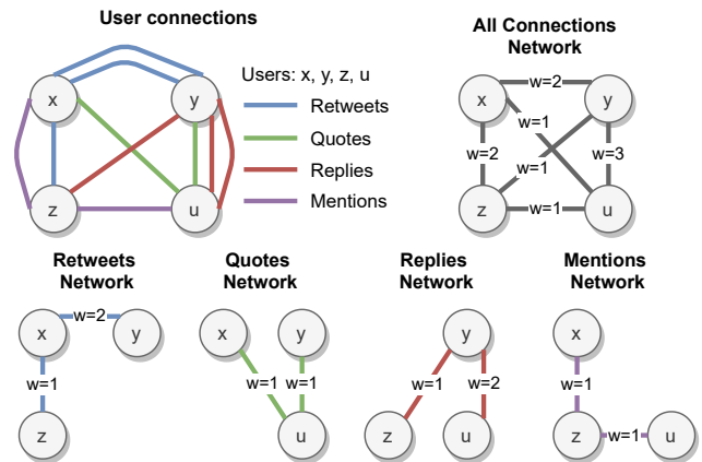
Fig. 2. Networks created from the different user connections.
